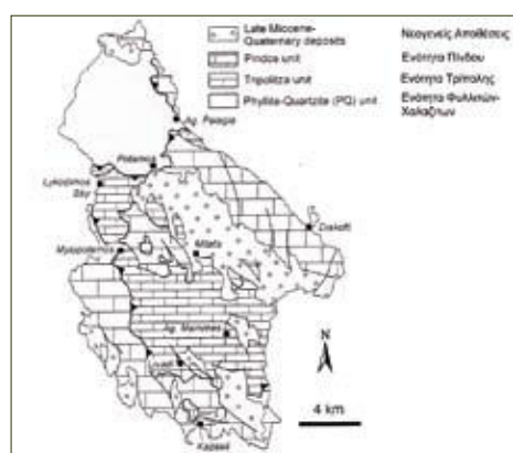
Figure 2. Simplified geological map of Kythera. (Xypollas et al 2008).
